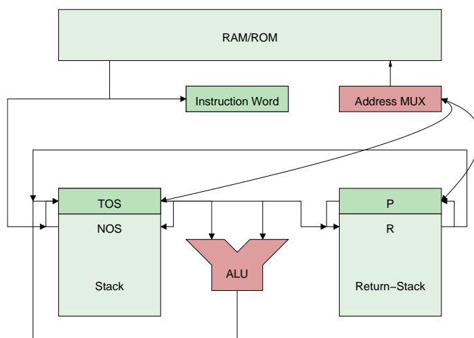
B16 small Block Diagram
